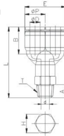
Diagram A - NPT & BSPT Tapered Thread
