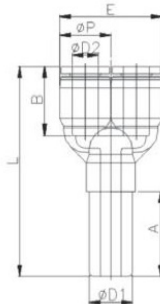
Diagram - Plug-In Reducer Y (PWJ)
