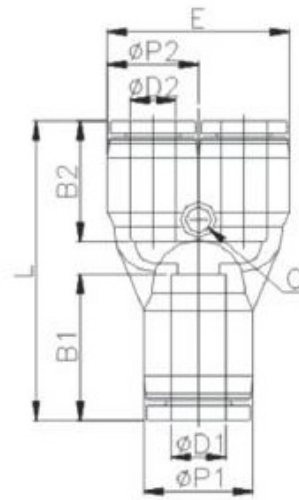
Diagram - Reducer Y (PW)
