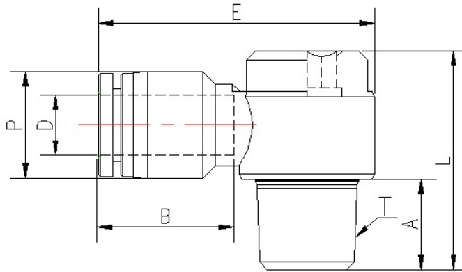
Diagram A - BSPT Tapered Thread
