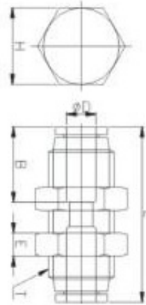
Diagram - Bulkhead Union (PMM)
