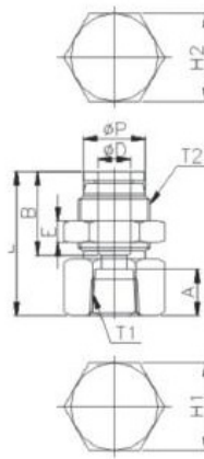
Diagram - NPT & BSPT Tapered Thread
