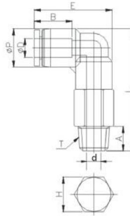
Diagram A - NPT & BSPT Tapered Thread
