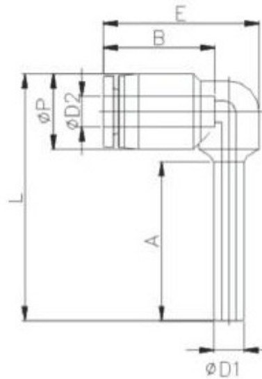
Diagram - Plug-In Elbow (PLJ)
