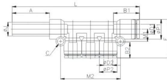
Diagram - Plug-In Reducer Triple Branch Union (PKJ)
