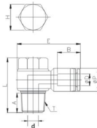
Diagram A - NPT & BSPT Tapered Thread
