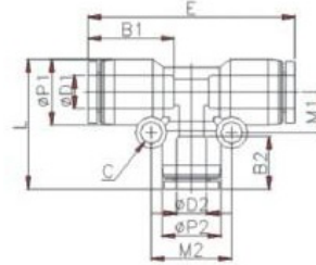
Diagram - Reducer Tee (PGT)
