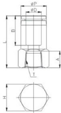
Diagram - Female Straight (PCF)
