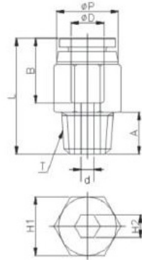
Diagram A - NPT & BSPT Tapered Thread
