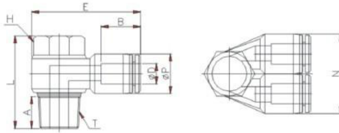
Diagram A - NPT & BSPT Tapered Thread
