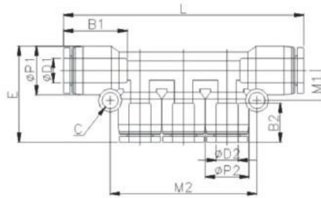
Diagram - Reducer Triple Branch Union (PKG)
