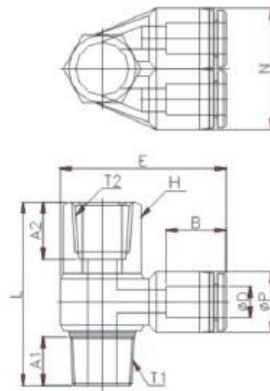
Diagram A - NPT & BSPT Tapered Thread
